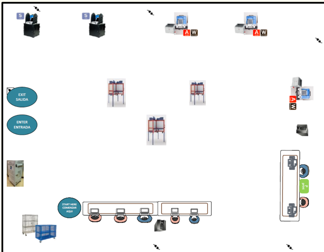
ii) Sample design of Voter Center layout with two Verity Scan (ballot scanner)
